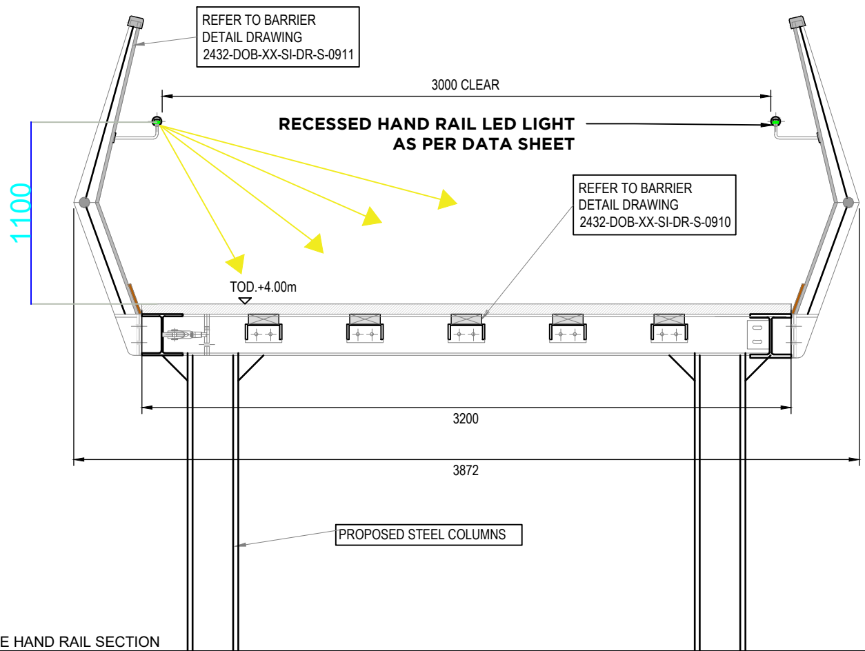
FIG 1: BRIDGE HAND RAIL SECTION
