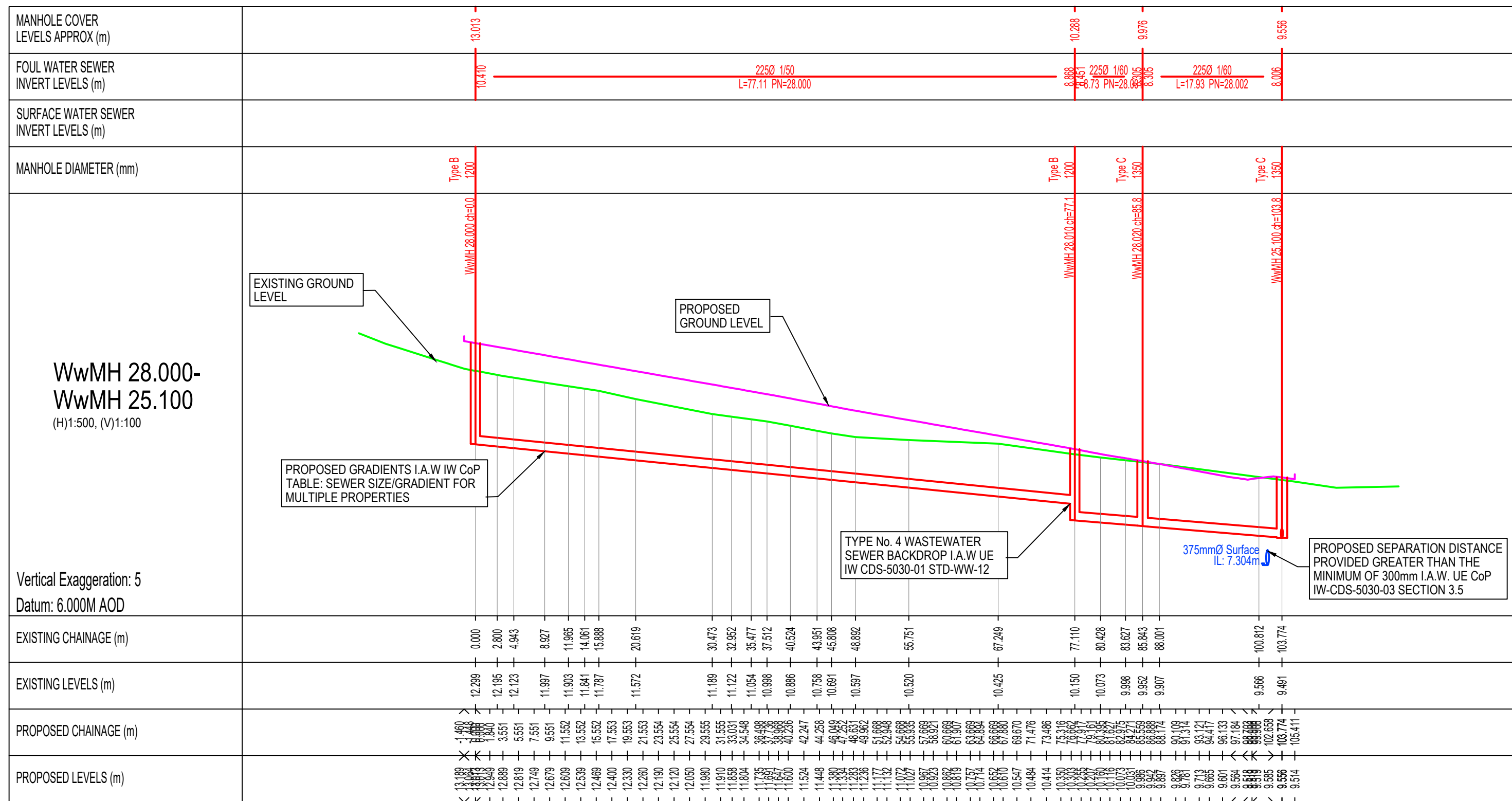
PROPOSED LONGITUDINAL SECTION WwMH 28.000- WwMH 25.100 SCALE 1:500
