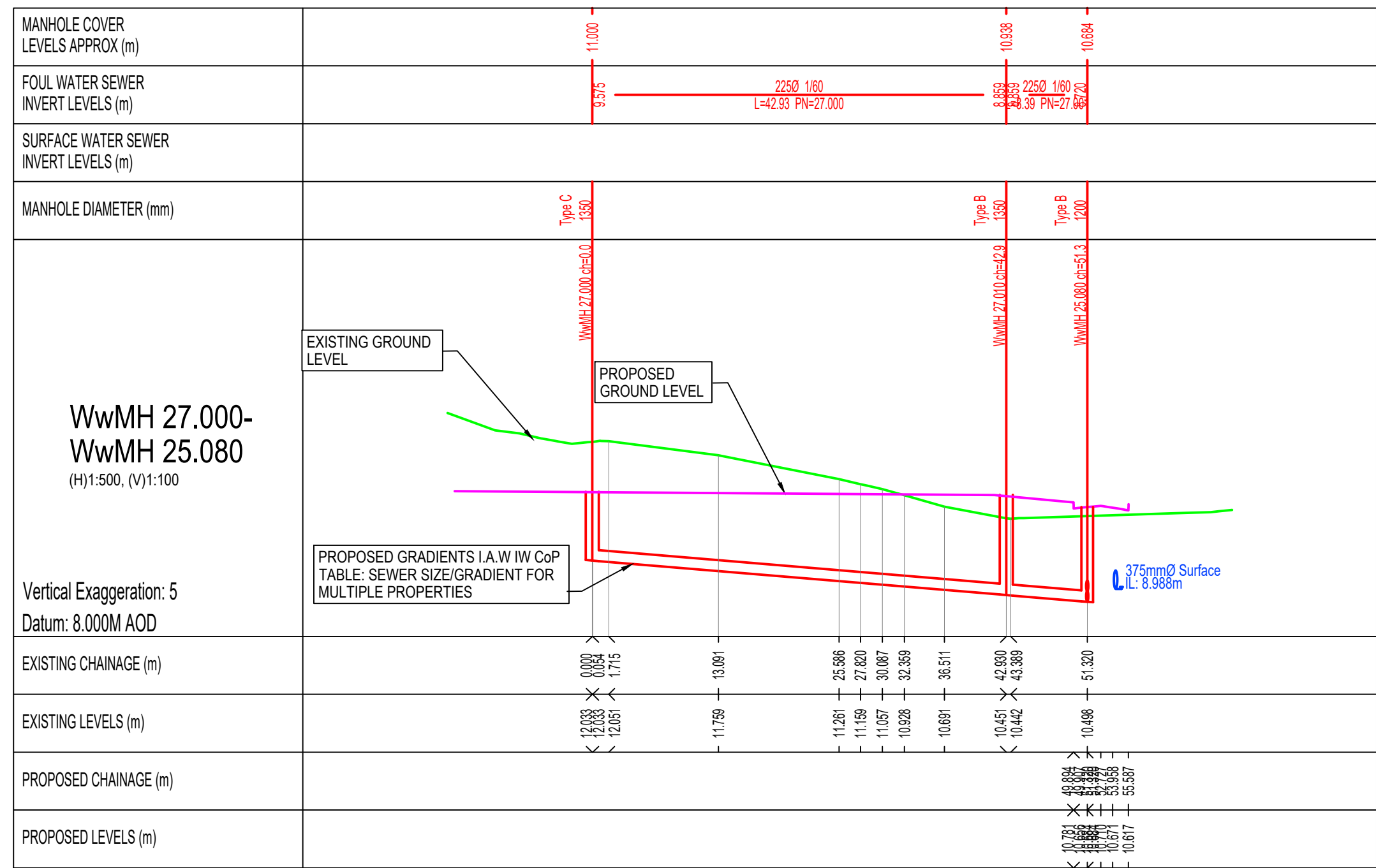
PROPOSED LONGITUDINAL SECTION WwMH 27.000- WwMH 25.080 SCALE 1:500
