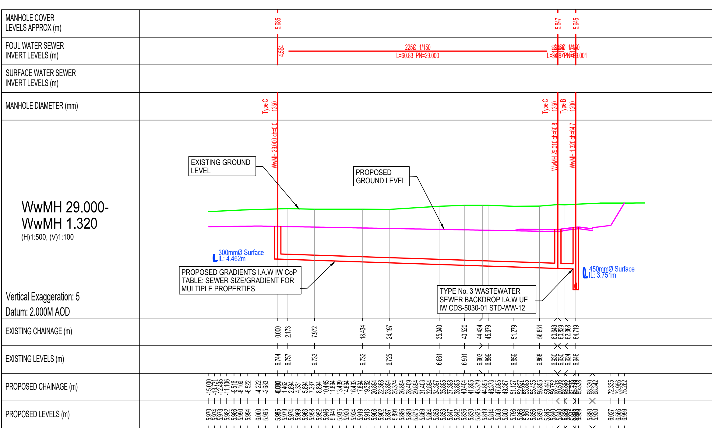
PROPOSED LONGITUDINAL SECTION WwMH 29.000- WwMH 1.320 SCALE 1:500
