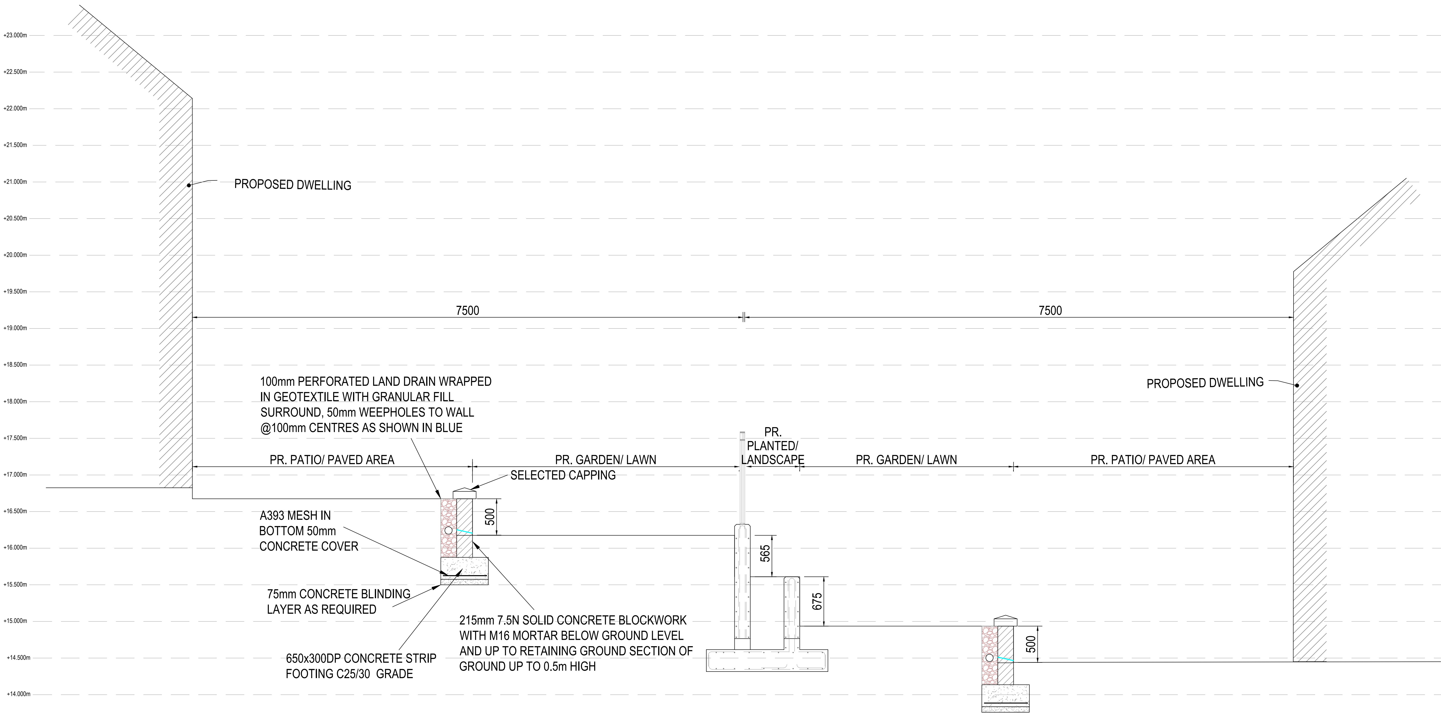
PROPOSED SECTION B-B SCALE: 1:25
