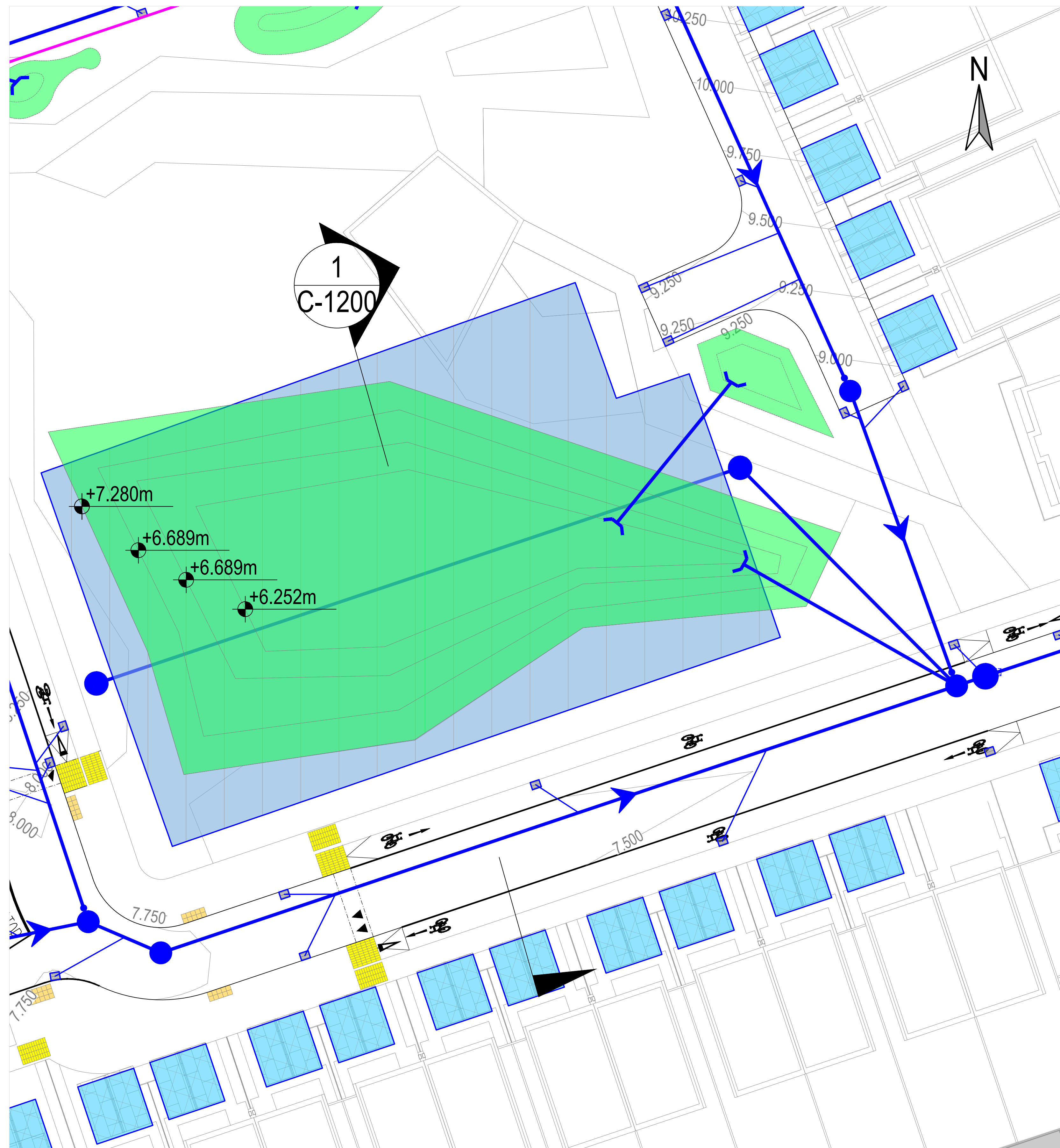
RETENTION POND PLAN SCALE 1:200
