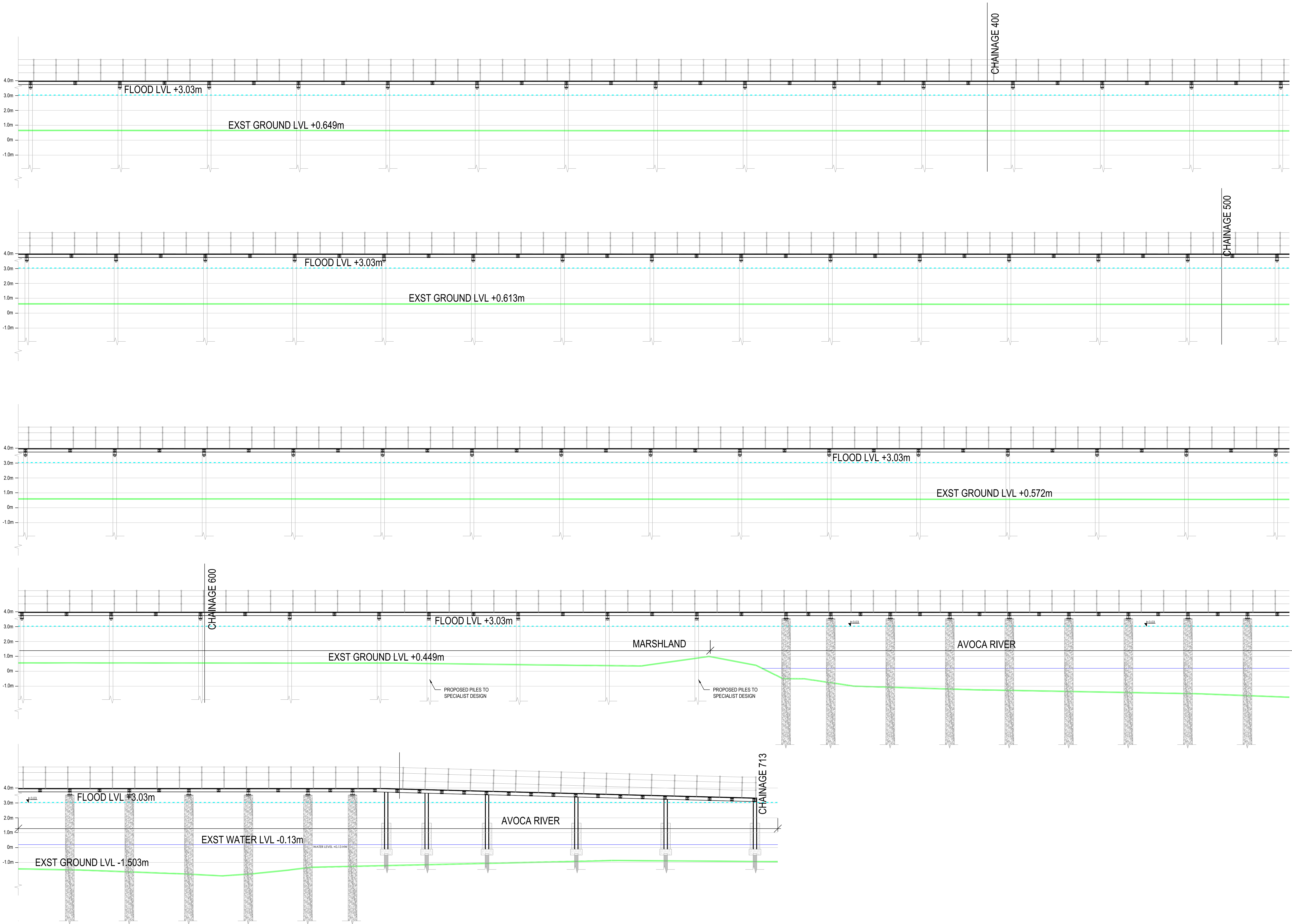
SECTION E-E TYPICAL LONG SECTION THROUGH PROPOSED BOARDWALK SCALE 1:100
