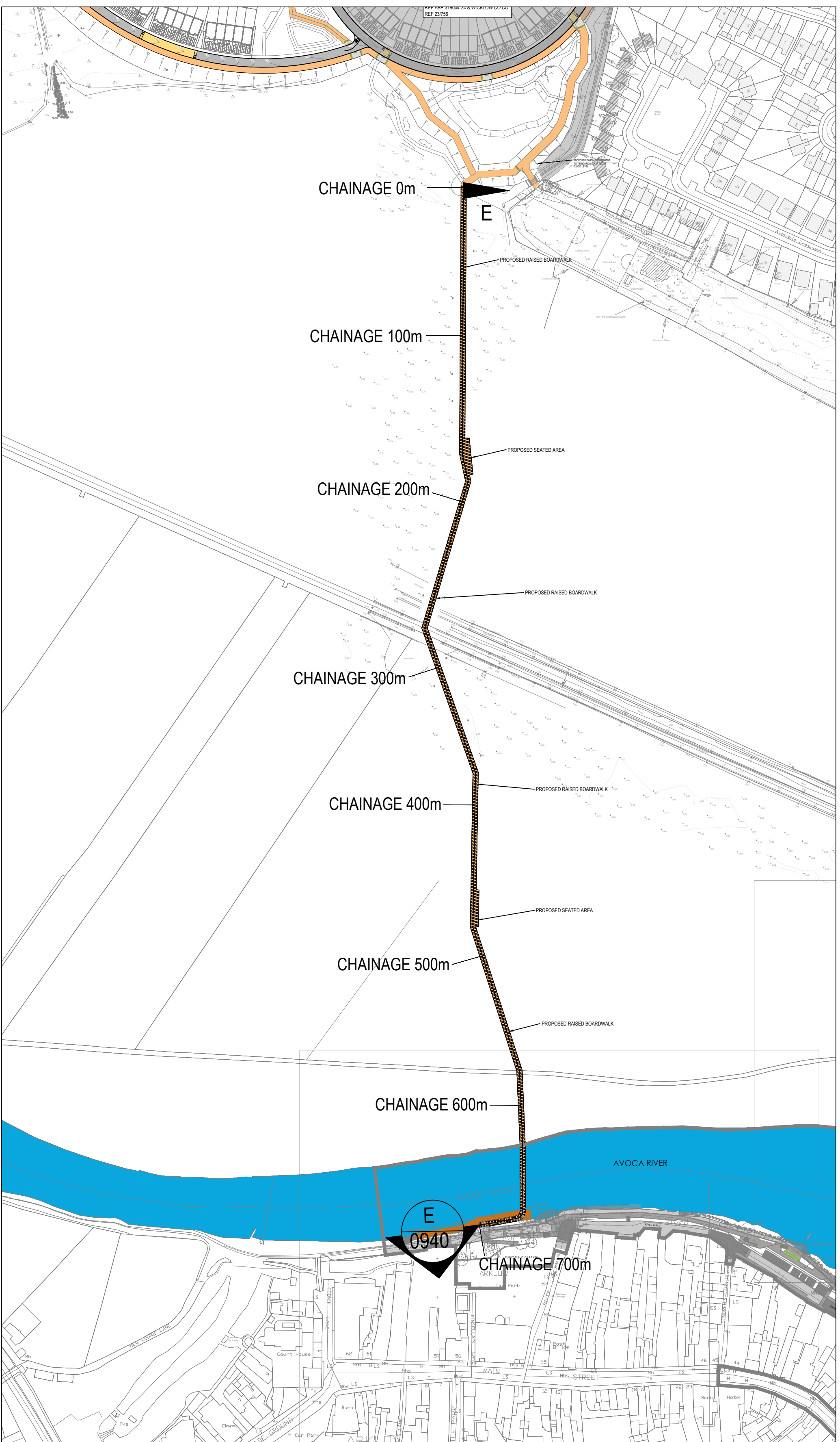
SITE KEY PLAN SCALE 1:2000
