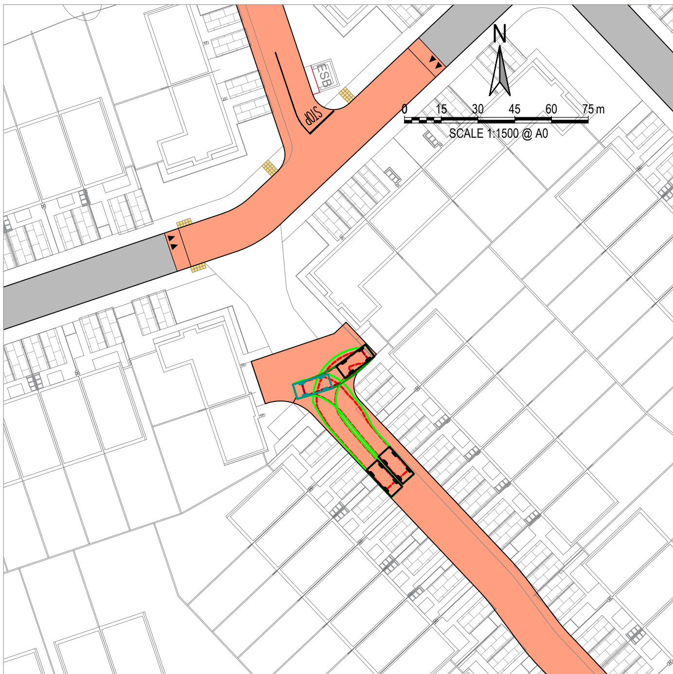
6 4x4 VEHICLE AT HAMMERHEAD Scale 1:500
