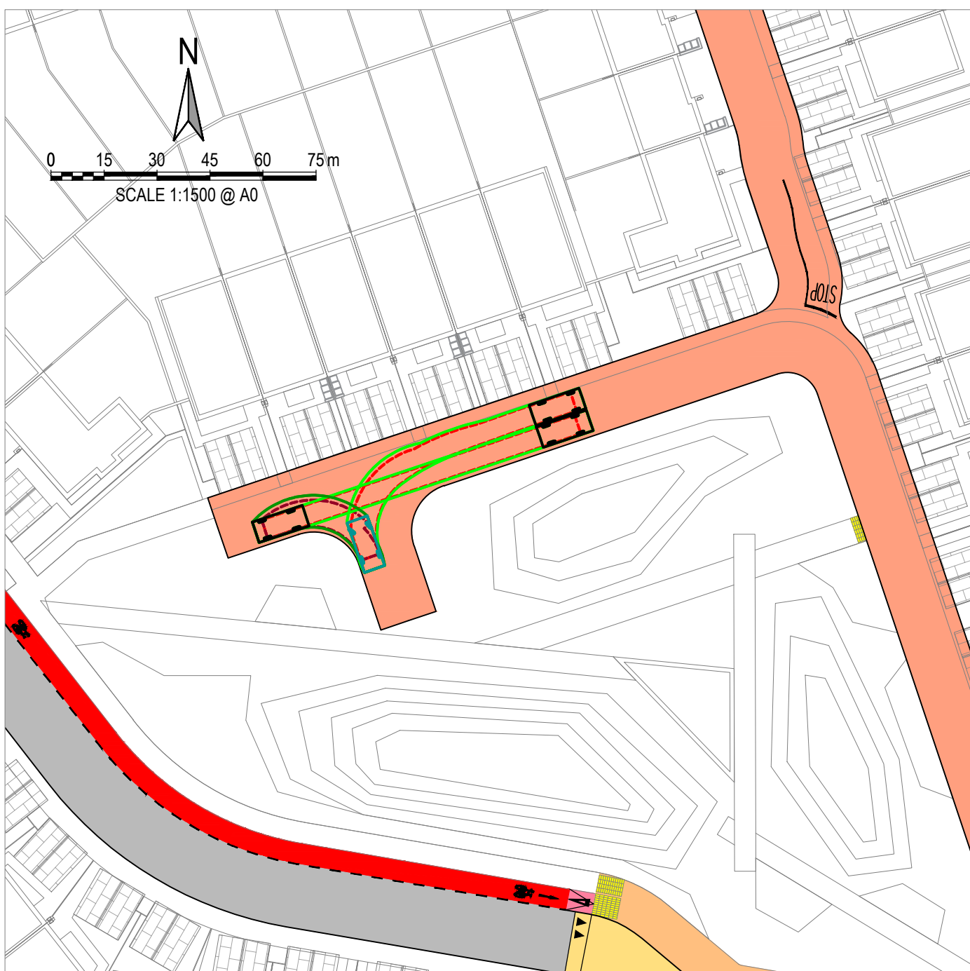
10 4x4 VEHICLE AT HAMMERHEAD Scale 1:500
