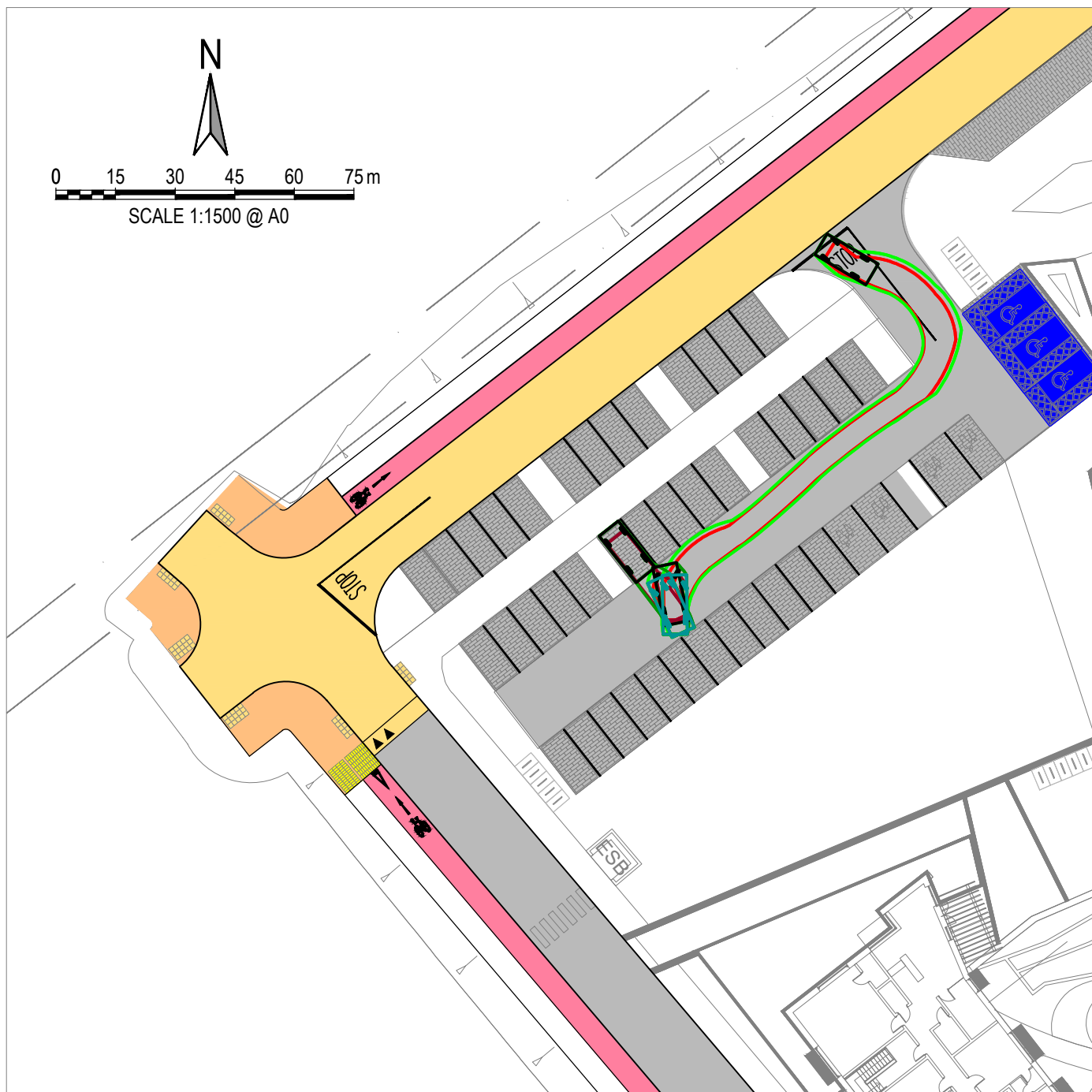
7 4x4 VEHICLE AT LOCAL CENTRE PARKING Scale 1:500
