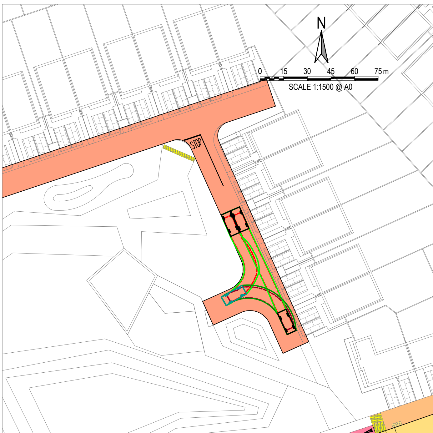
9 4x4 VEHICLE AT HAMMERHEAD Scale 1:500
