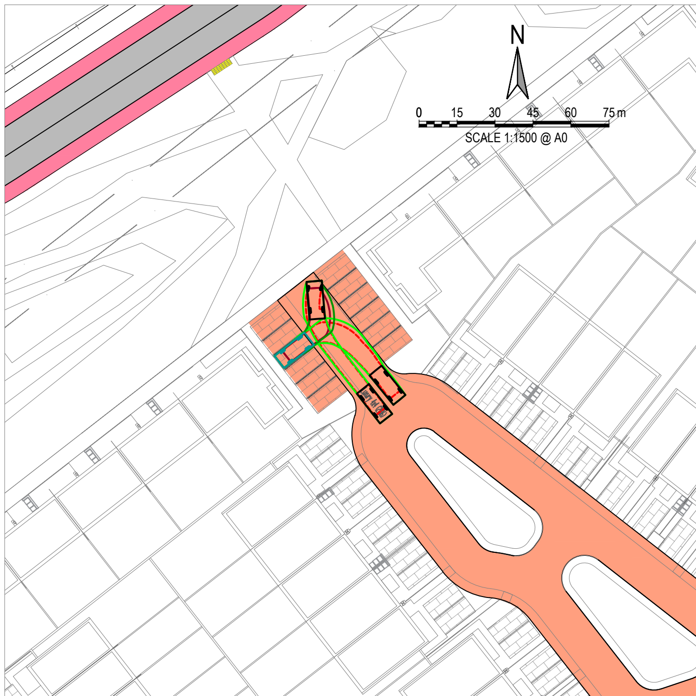
8 4x4 VEHICLE AT GROUP PARKING Scale 1:500
