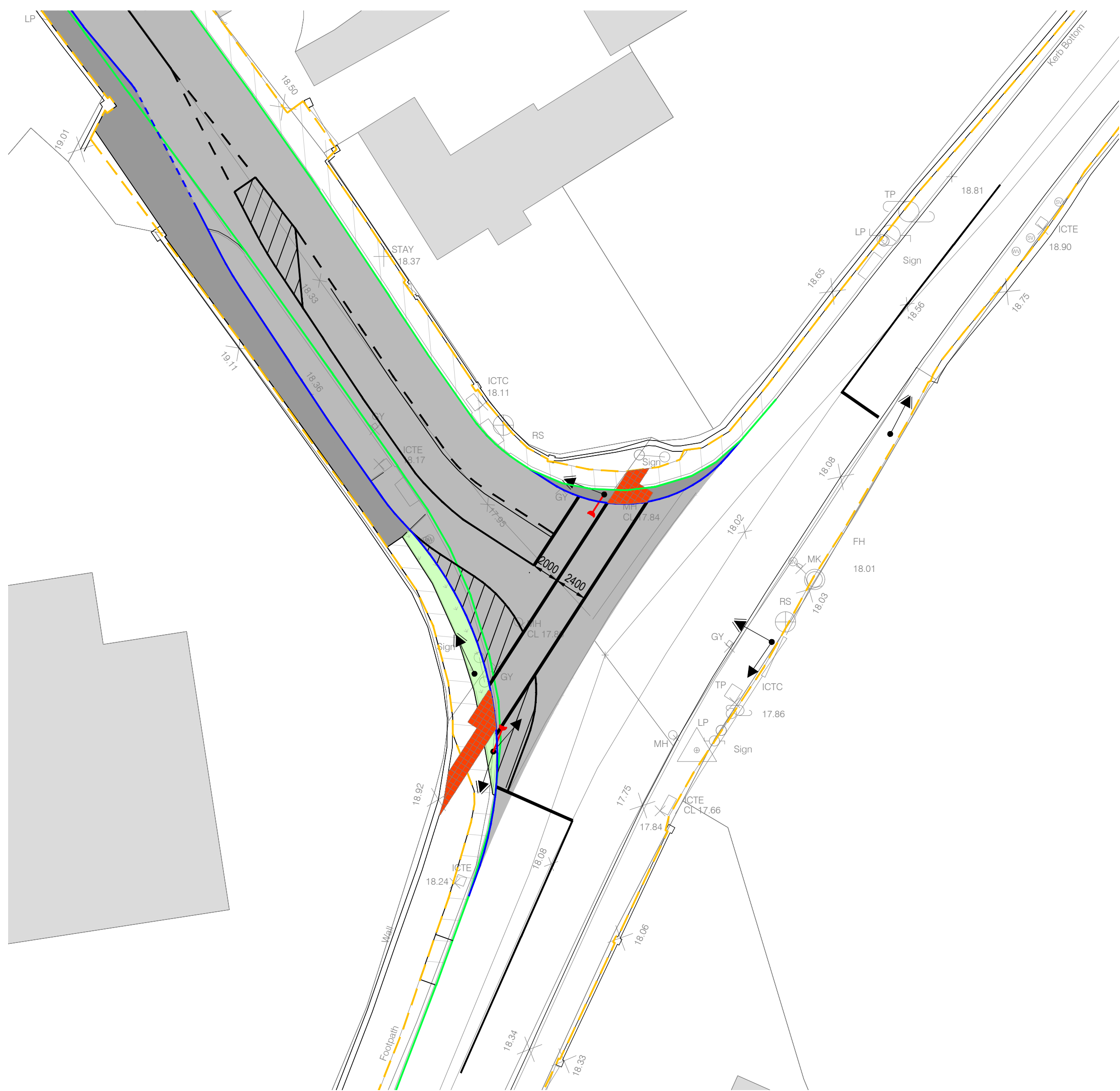
VEHICLE TRACKING - REFUSE ACCESS JUNCTION ENTRY SCALE 1:250
