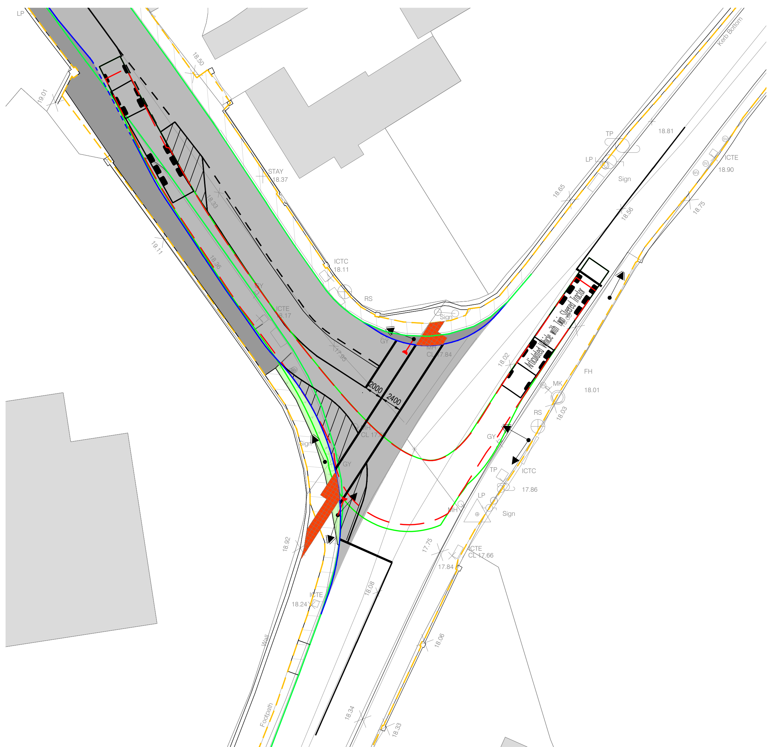
VEHICLE TRACKING - HGV ACCESS JUNCTION ENTRY SCALE 1:250
