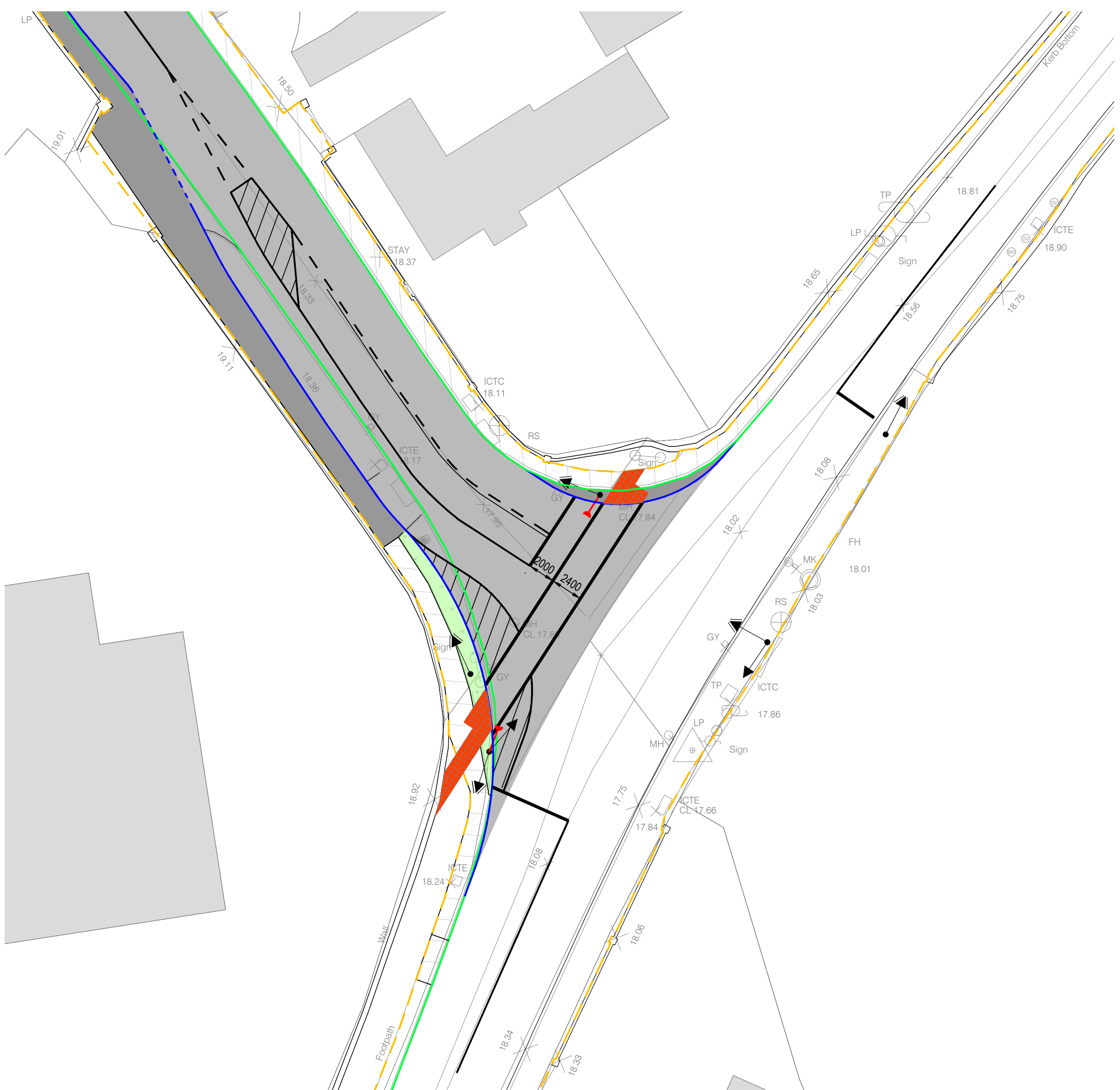
VEHICLE TRACKING - HGV ACCESS JUNCTION EXIT
