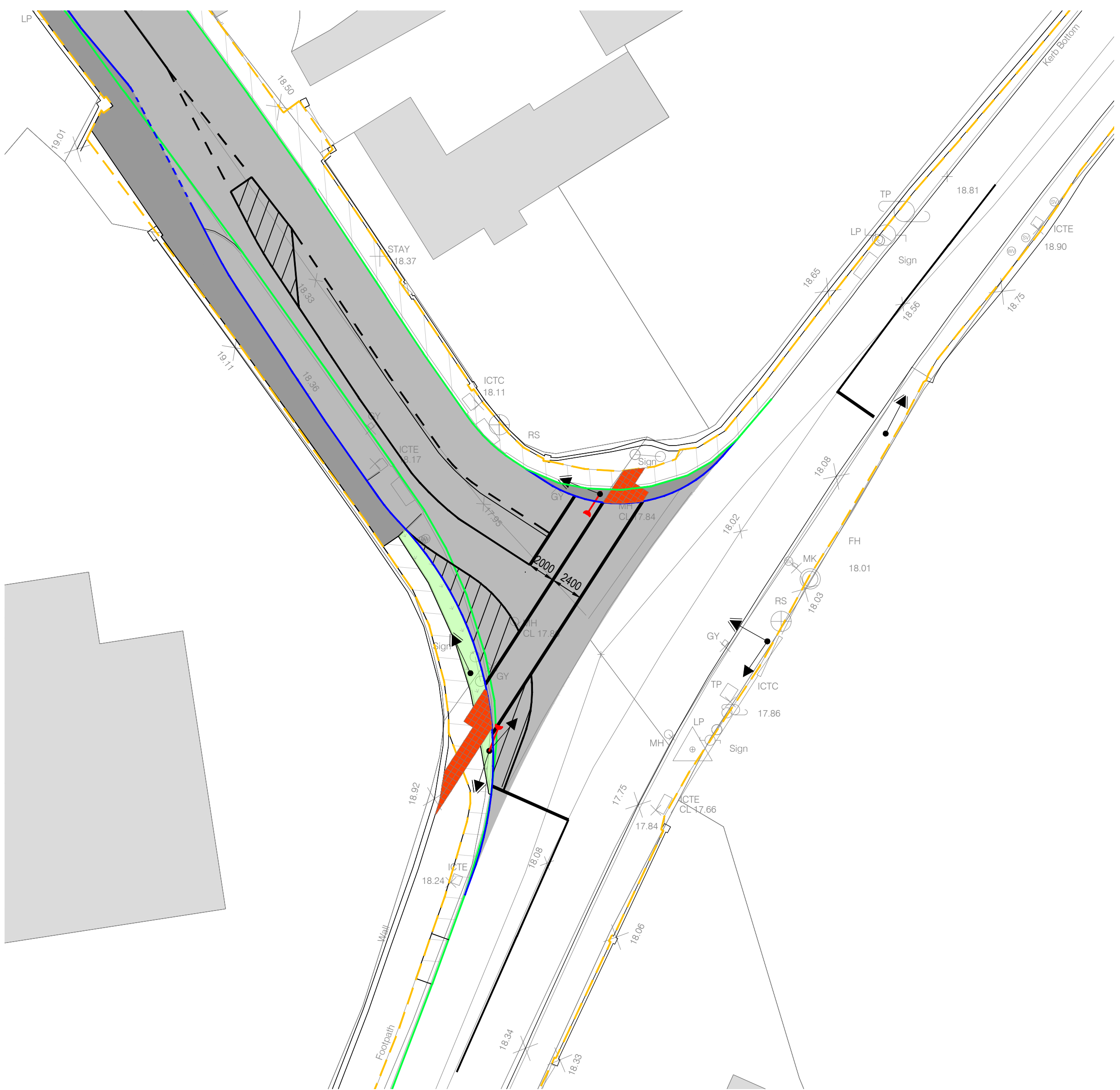
VEHICLE TRACKING - REFUSE ACCESS JUNCTION EXIT
