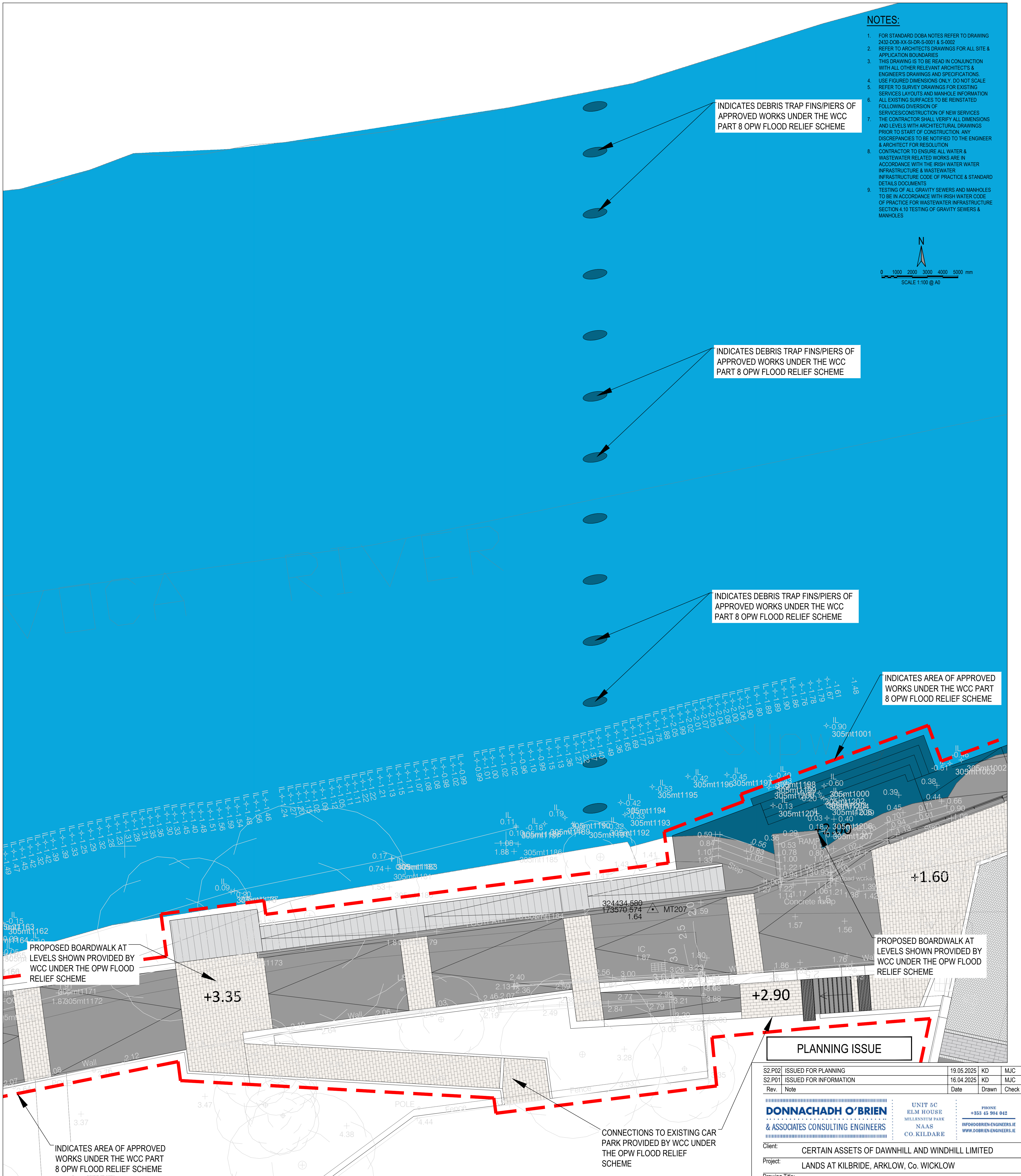
PROPOSED SOUTHERN BANK BOARDWALK AS PART OF THE APPROVED WICKLOW COUNTY COUNCIL PART 8 APPLICATION FOR THE OPW FLOOD RELIEF SCHEME SCALE 1:100
