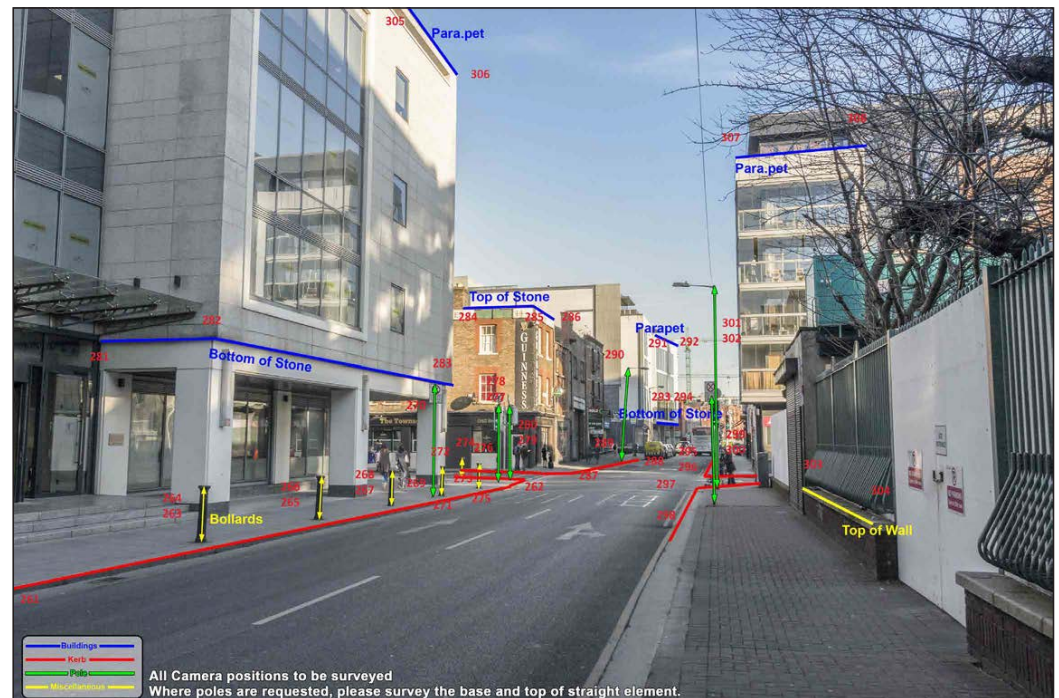
Fig.8: Fixed reference points fully surveyed and numbered.
