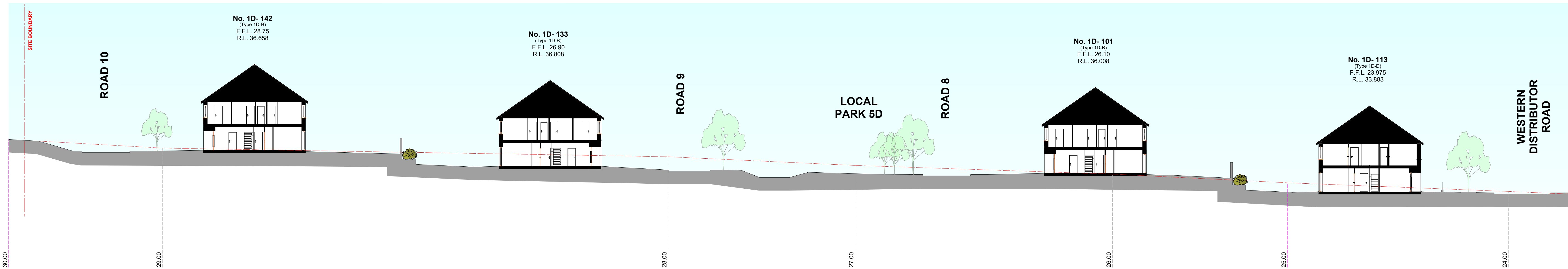
SITE SECTION H Scale 1:200
