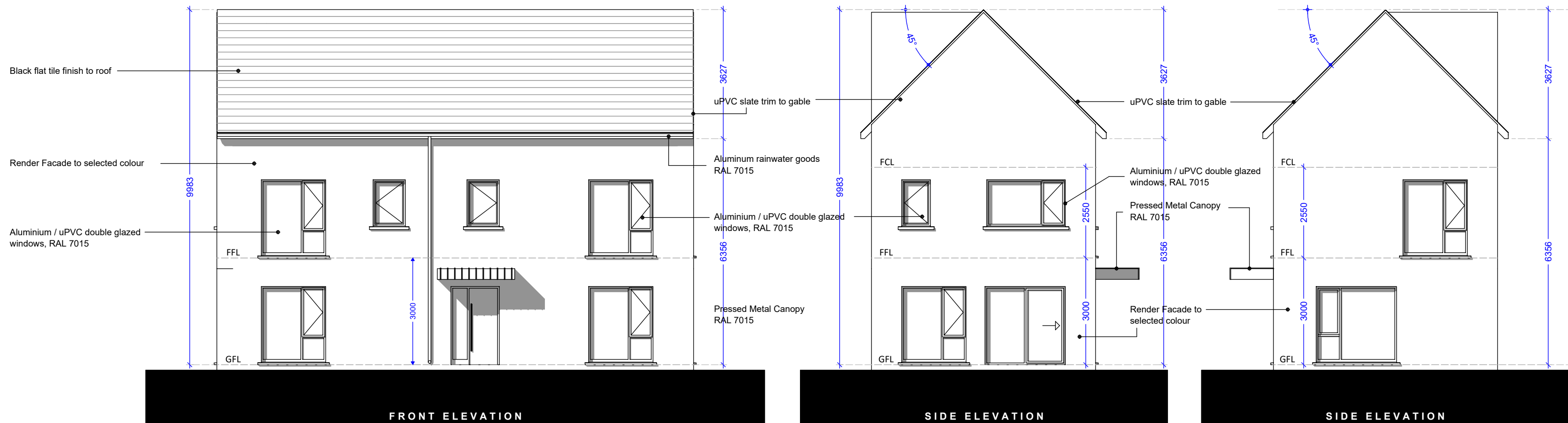
TYPE 1D-A with RENDER FACADE House Nos. 1, 8, 28, 106, 148, 164.
