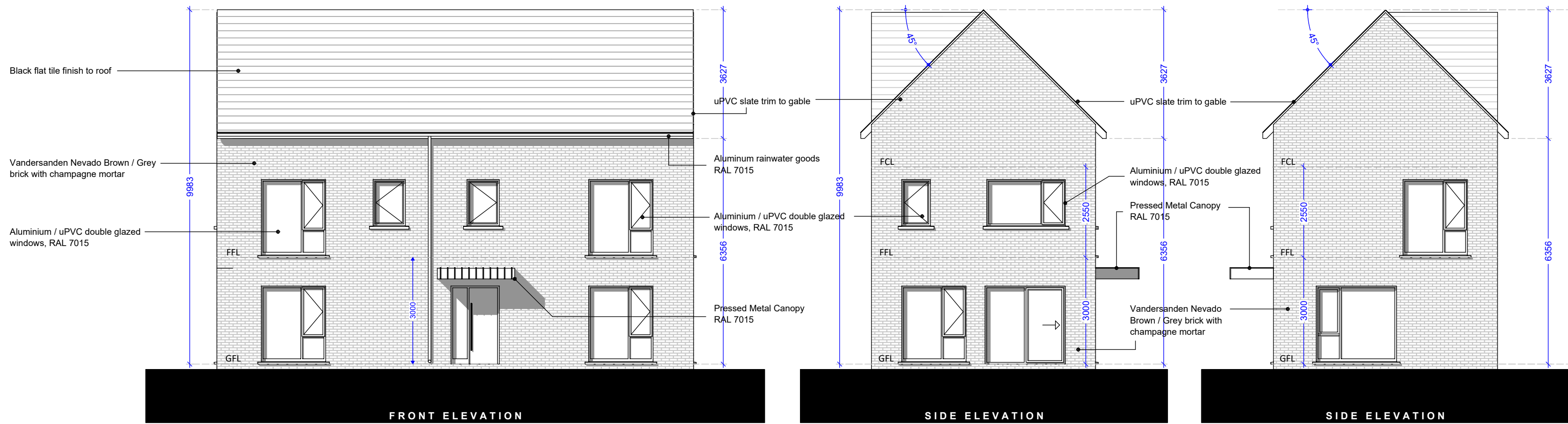
TYPE 1D-A with BRICK FACADE House Nos. 19, 29, 38, 55, 56, 72, 82, 89, 93, 100, 107, 115, 128, 137, 138, 147, 155.
