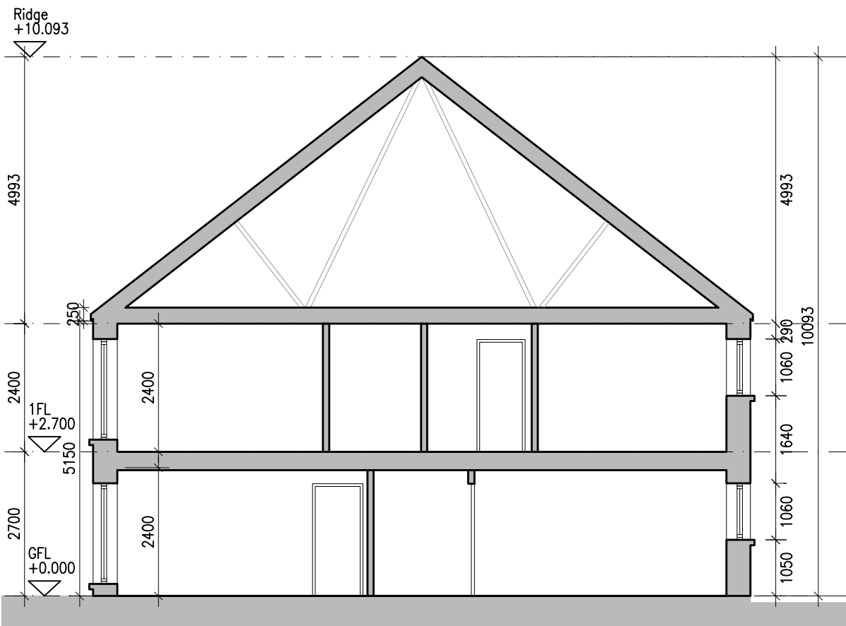
7 Type H1 - Section AA 1:100@A1 4 BED HOUSE
