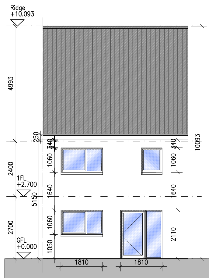
06 Type H1 - Rear Elevation 1:100@A1 4 BED HOUSE
