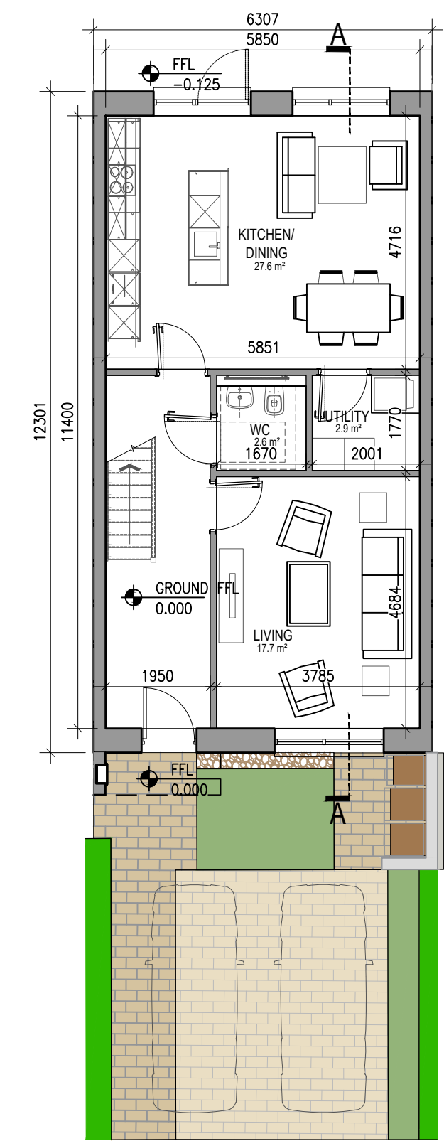
01 Type H1 - Ground Floor Plan 1:100@A1 4 BED HOUSE
