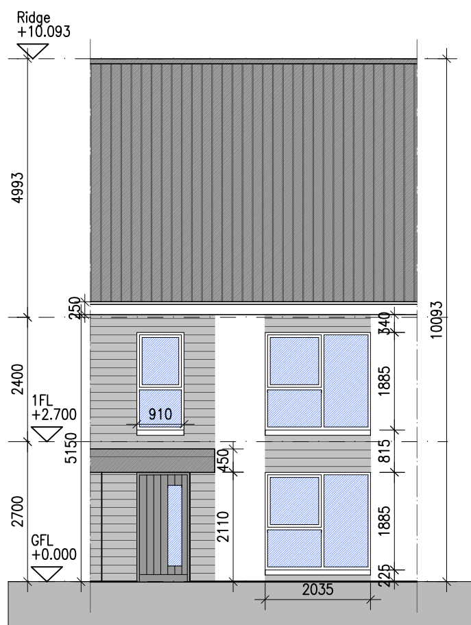
04 Type H1 - Front Elevation [Character Area 1B] 1:100@A1 4 BED HOUSE
