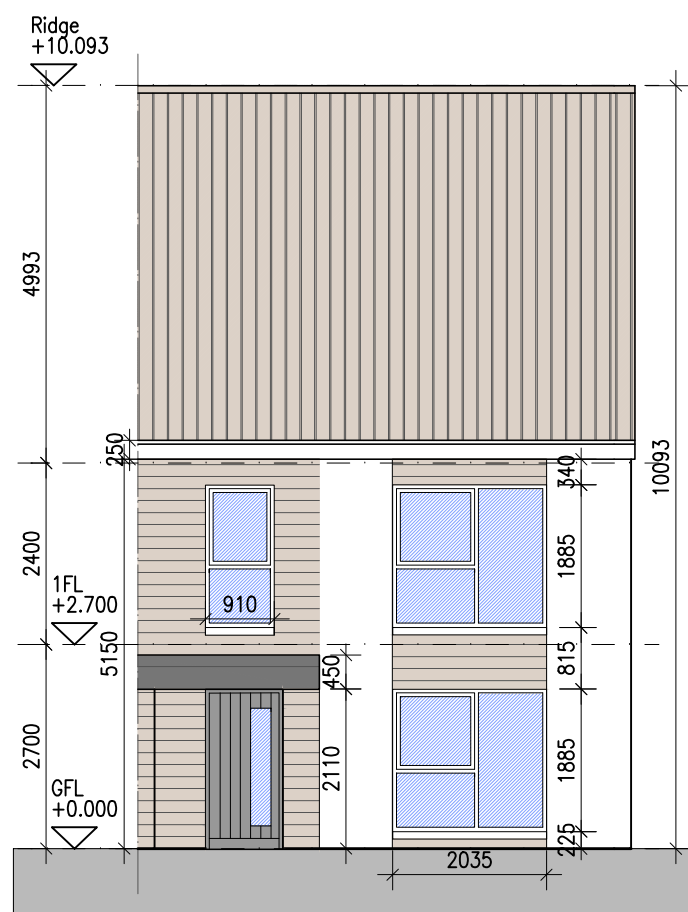
05 Type H1 - Front Elevation [Character Area 1C] 1:100@A1 4 BED HOUSE
