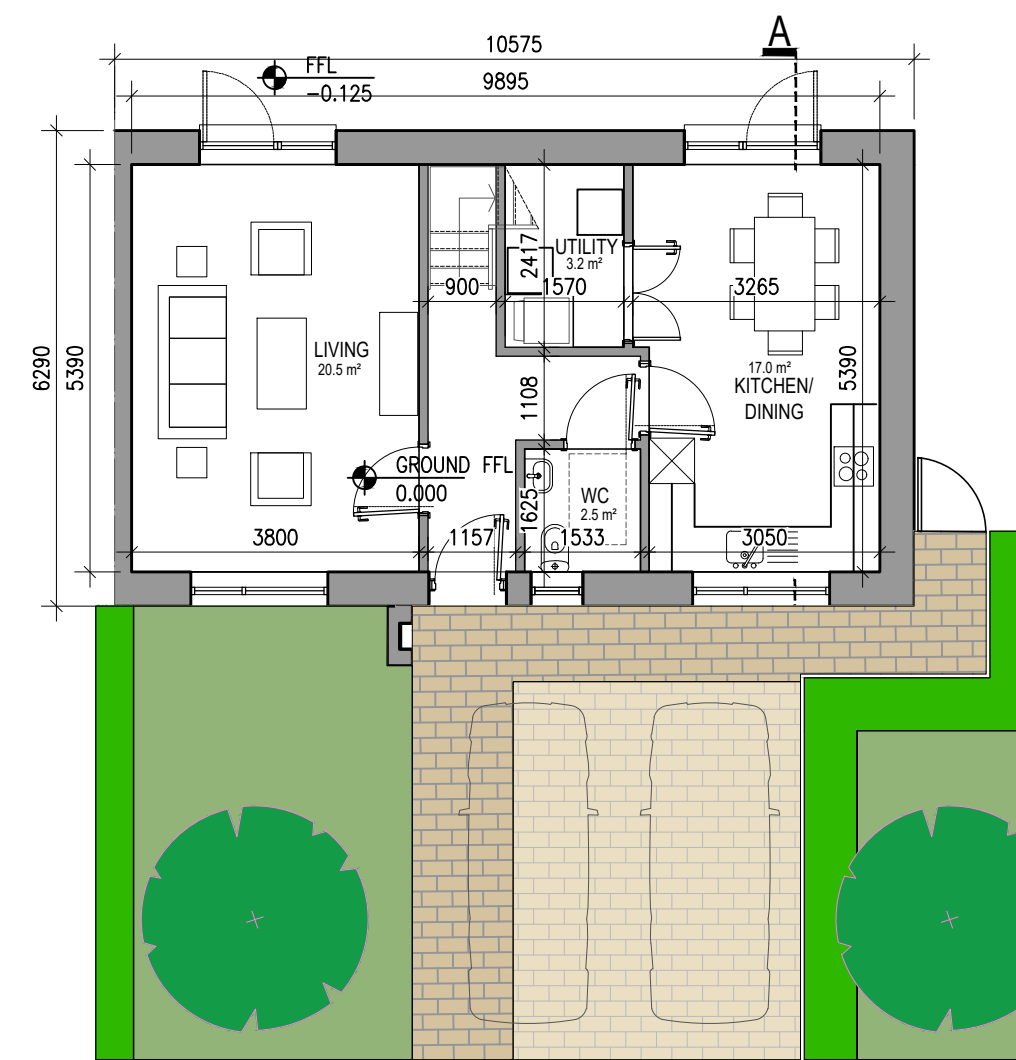
08 Type F2 - Ground Floor Plan 207 1:100@A1 3 BED HOUSE
