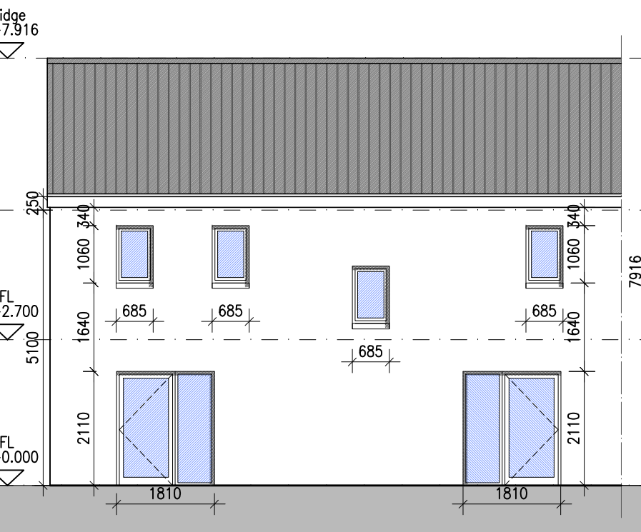
13 Type F2 - Rear Elevation 207 1:100@A1 3 BED HOUSE
