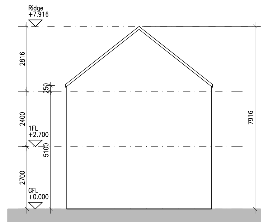
15 Type F2 - Side Elevation 207 1:100@A1 3 BED HOUSE
