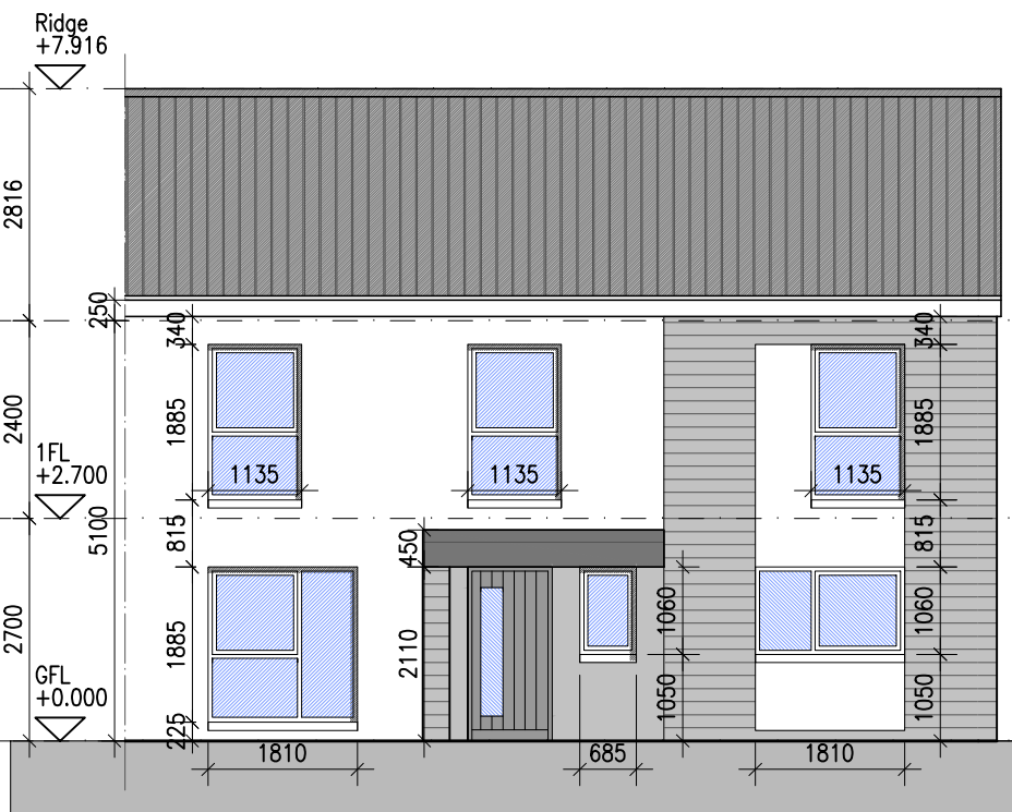
11 Type F2 - Front Elevation [Character Area 1B] 207 1:100@A1 3 BED HOUSE
